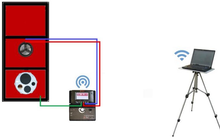
Fig. 2.3: Example of set-up for the field calibration check with the measuring system BlowerDoor MiniFan with digital pressure gauge DG-1000 (here: WiFi connection). The use of DG-700 gauge and other communication links are possible.
