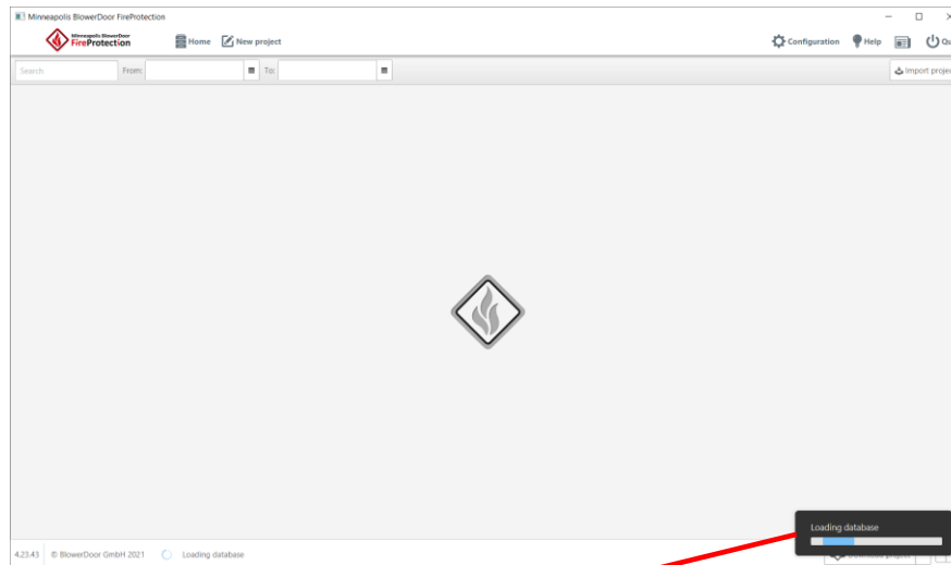
Fig. 4.10: Home screen
