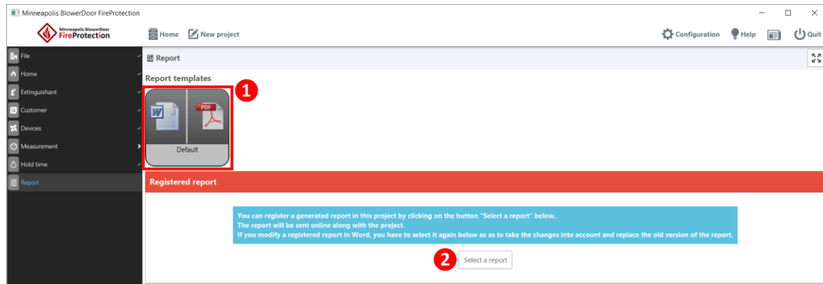
Fig. 6.48: Report screen
